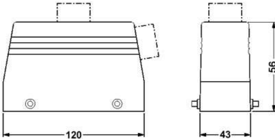
Dimensioned drawing
