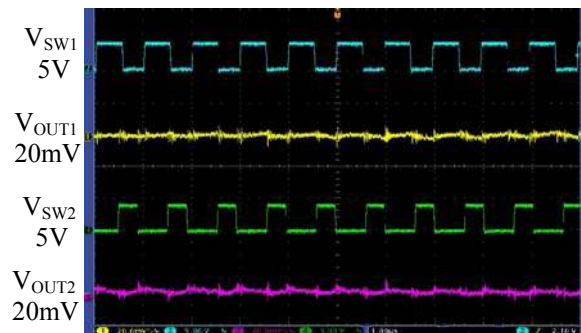
Time 1μs/div
