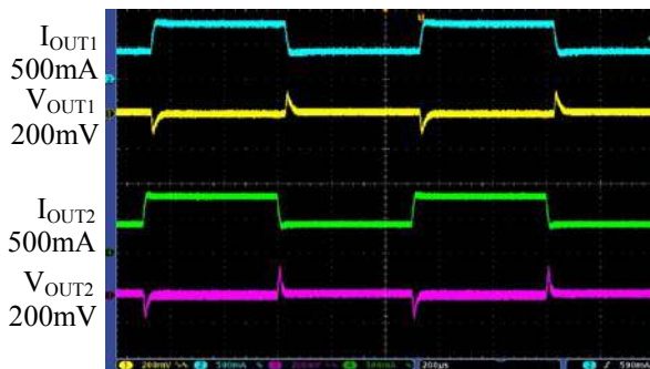
Time 200μs/div
