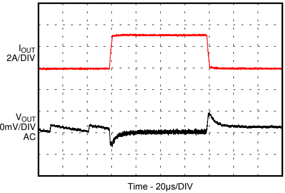
Figure 8-21. Load Transient
