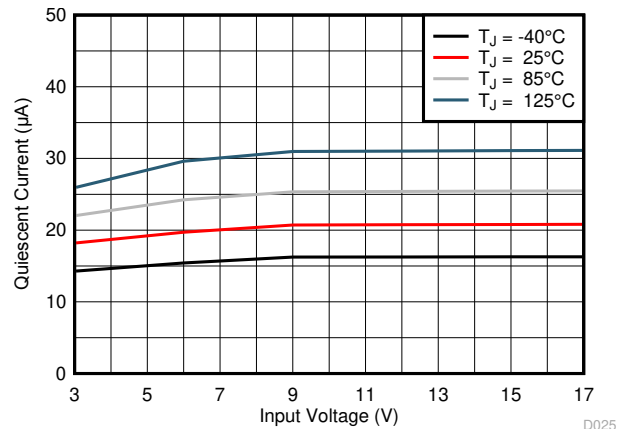
Figure 6-2. Quiescent Current
