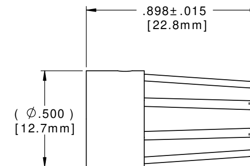
BACKSHELL, LONG MAT'L: NYLON, BLACK
