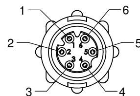
FACE VIEW 18982-6SG-5XX 6 POSITION B-KEY
