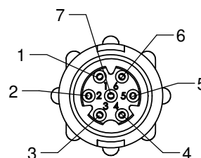
FACE VIEW 18982-7SG-5XX 7 POSITION A-KEY
