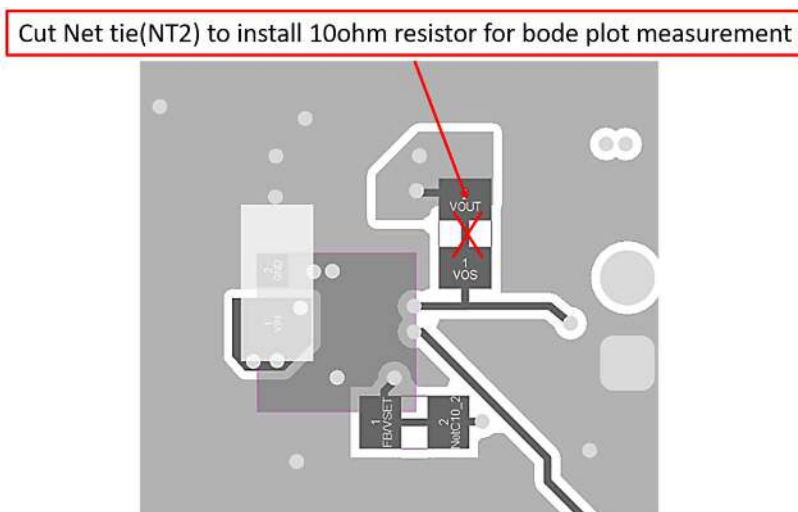
Figure 3-2. Bode Plot Measurement Board Modification
