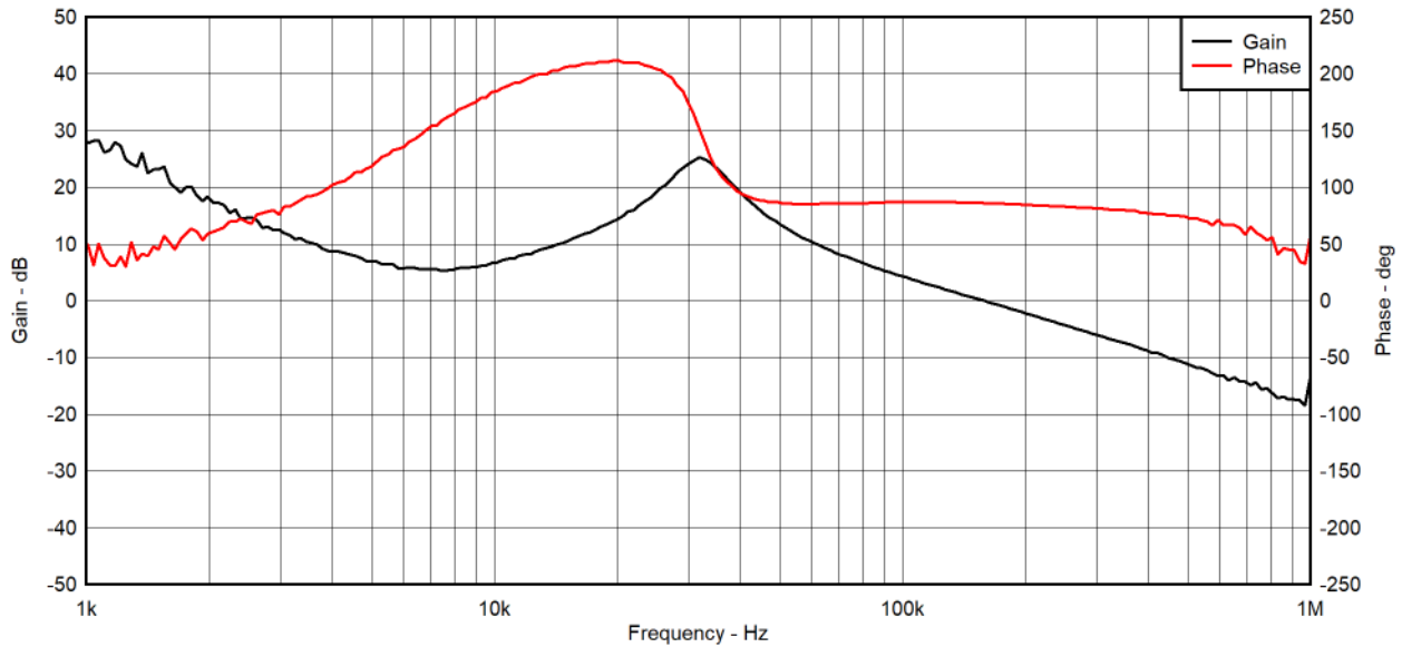
Figure 5-4. Loop Response, Forced PWM VSET, V_{IN} = 12\text{ V} , V_{OUT} = 3.3\text{ V} , I_{OUT} = 300\text{ mA}
