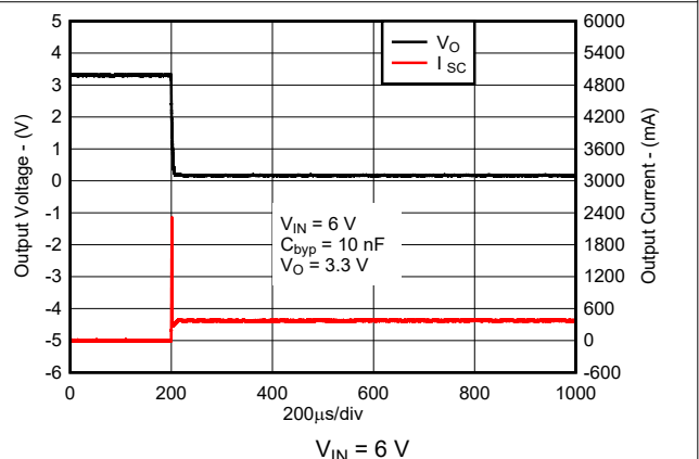
Figure 6-10. Short-Circuit Current vs Time for New Chip
