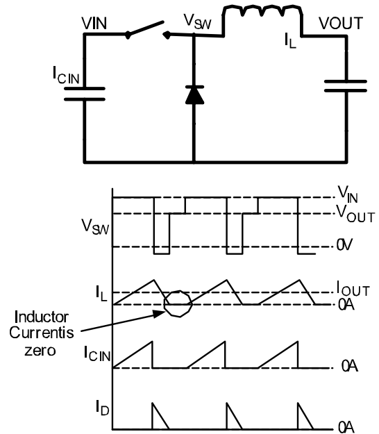
Figure 5. Discontinuous Operation
