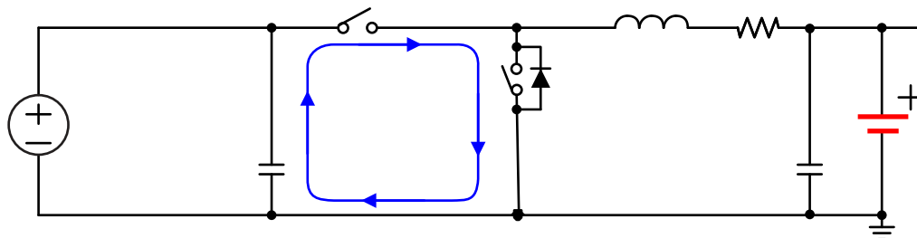
Figure 51. High Frequency Current Path
