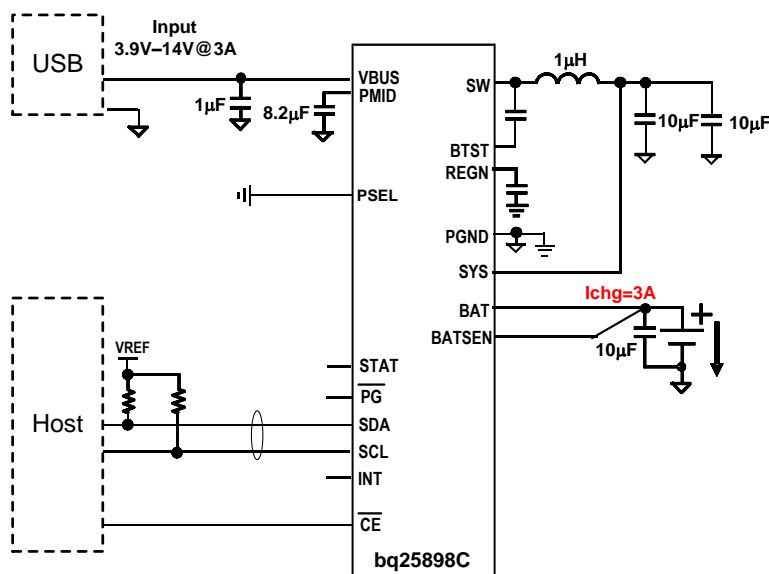
Figure 40. bq25898C Application Diagram as Slave Charger
