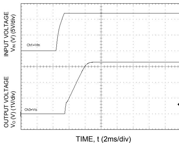
Fig-26. Typical Start-up Using Input Voltage (VIN = 12V, Io = Io,max).
