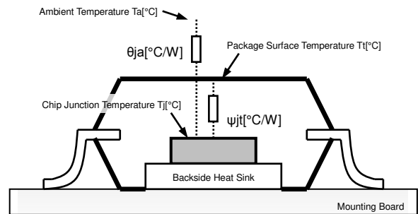
Figure 77. Thermal Resistance Model of Backside Exposed Package with Heat Sink
