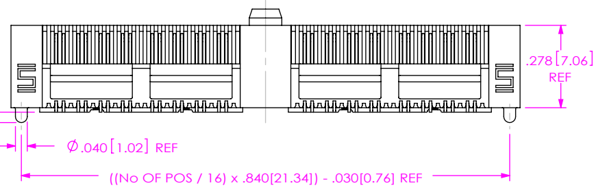
FIG 1 QFS-032-04.25-X-D-DP-A SHOWN
