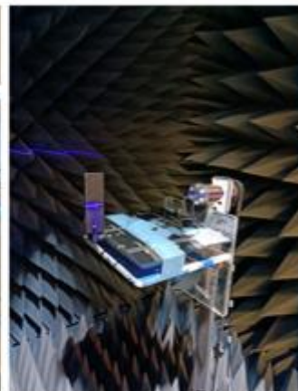
Chamber & VNA setup bent on the edge of a 30x30cm ground plane
