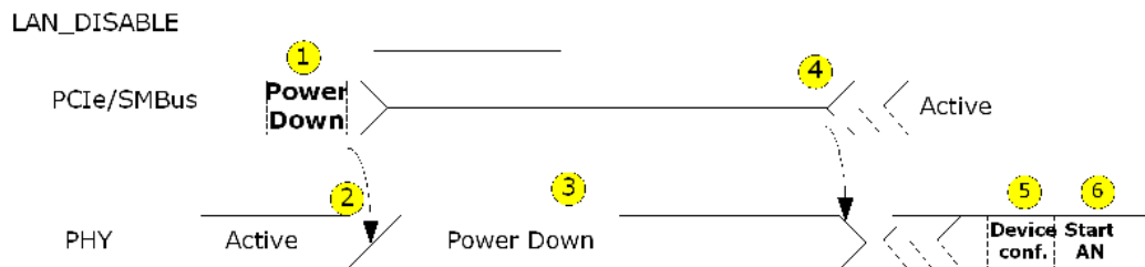
Figure 6. Power-Down Sequence
