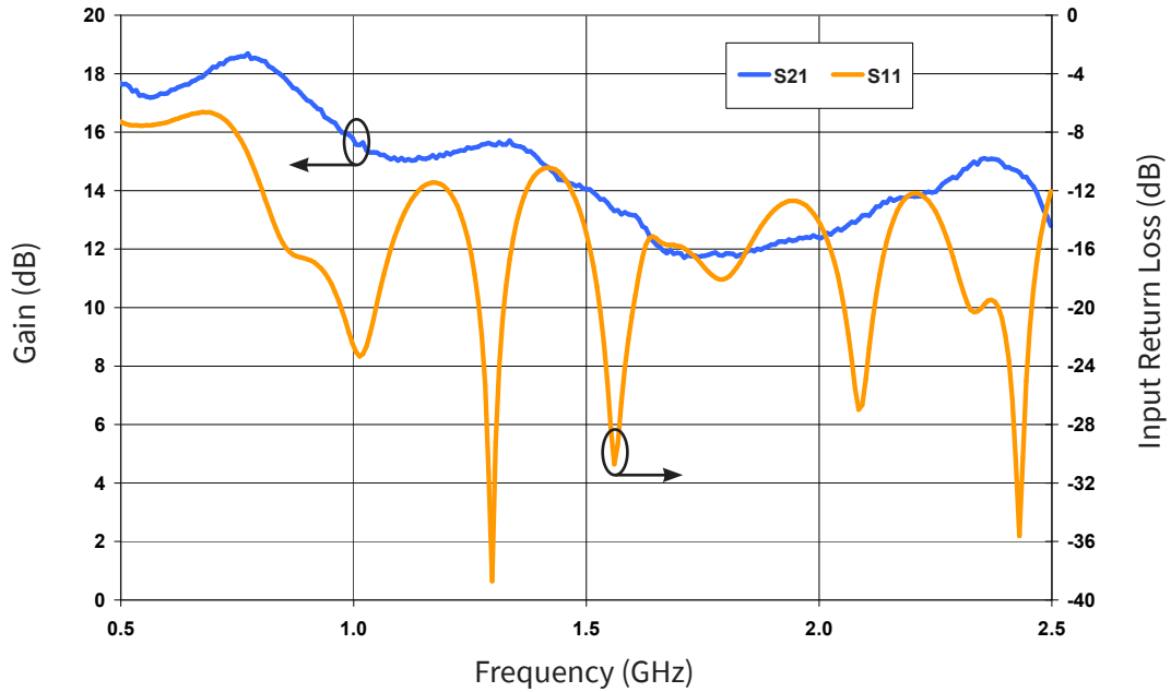
Gain and Input Return Loss vs Frequency from 0.5 GHz to 2.5 GHz in Broadband Amplifier Circuit CGH40090PP-AMP V_{DD} = 28\text{ V}, I_{DQ} = 1.0\text{ A}
