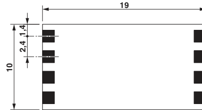
Dimensional drawing
