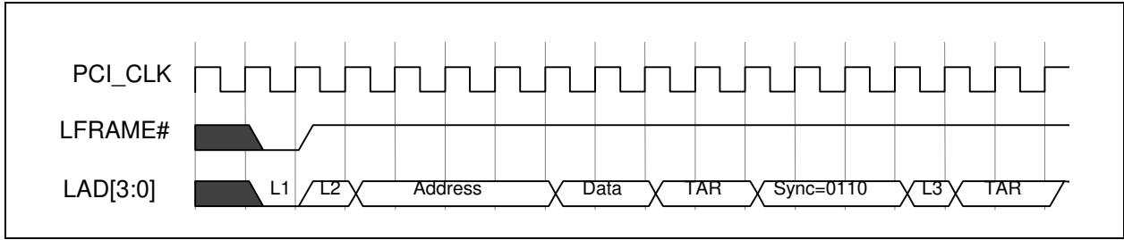
FIGURE 27-7: I/O WRITE
