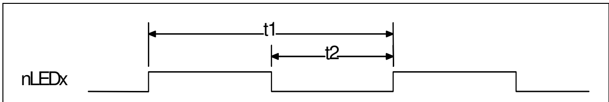
FIGURE 27-29: NLEDX TIMING
