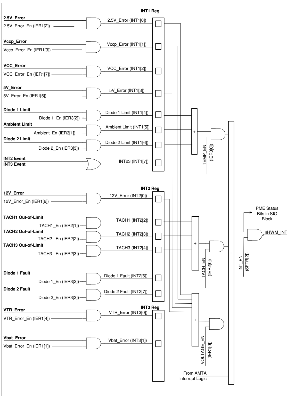
FIGURE 21-3: INTERRUPT CONTROL
