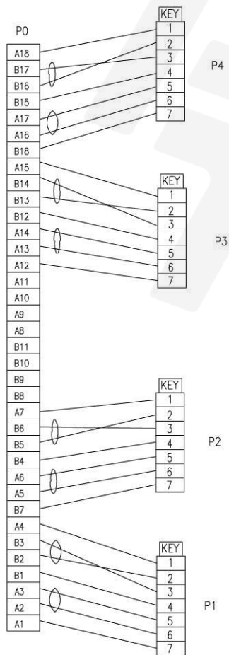
WIRING DIAGRAM
