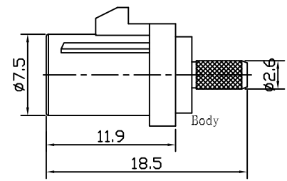
Plastic shell
