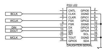
P22 (TOP) = SAMTEC - PIN: TSM-110-01-L-DV-P J22 (BOTTOM) = SAMTEC - PIN: SSW-110-22-F-D-VS-K
