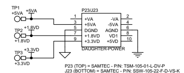
P23 (TOP) = SAMTEC - PIN: TSM-105-01-L-DV-P J23 (BOTTOM) = SAMTEC - PIN: SSW-105-22-F-D-VS-K
