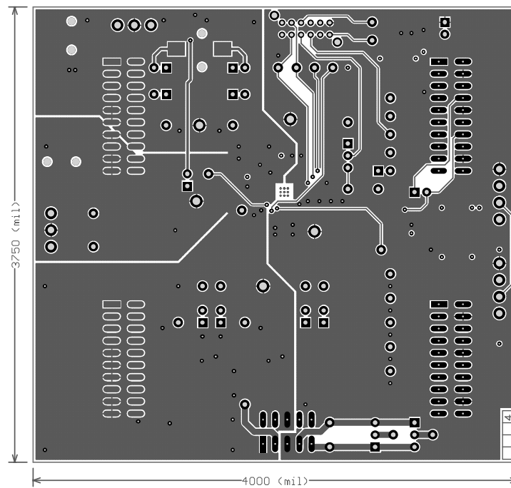
Figure 15. Bottom Layer
