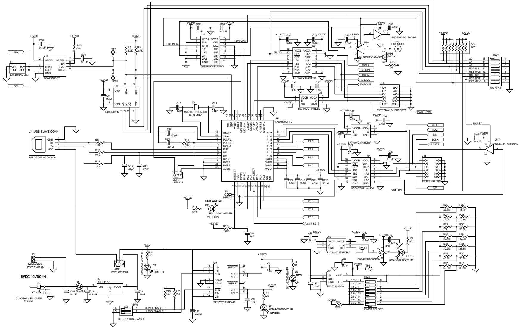
Figure 21. USB-MODEVM Schematic (Sheet 2 of 3)
