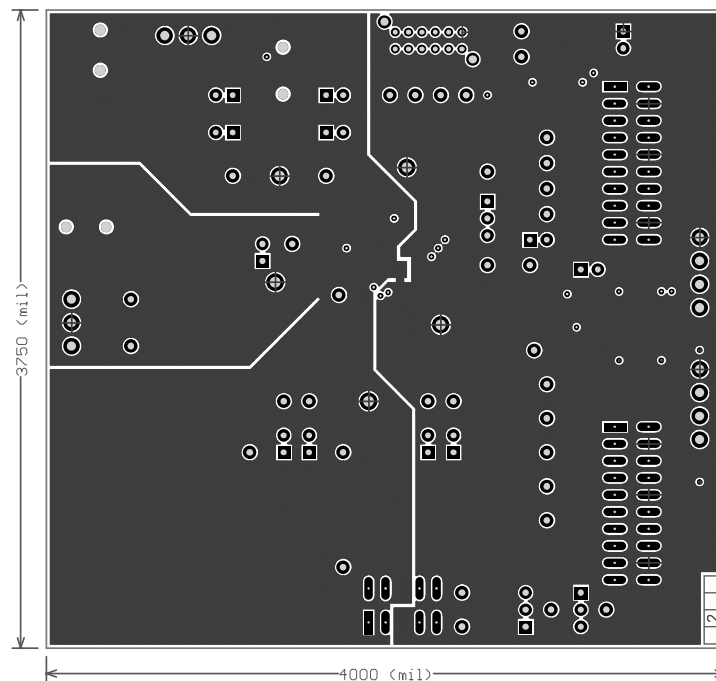
Figure 13. Mid-Layer 1
