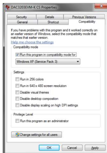
Figure 2. Compatibility Tab
