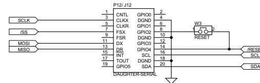
P12 (TOP) = SAMTEC - PIN: TSM-110-01-L-DV-P J12 (BOTTOM) = SAMTEC - PIN: SSW-110-22-F-D-VS-K
