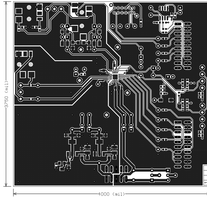
Figure 12. Top Layer
