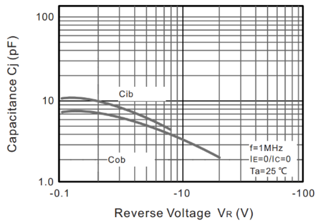
Fig.8 C_{ob}/C_{ib}-V_{CB}/V_{EB}
