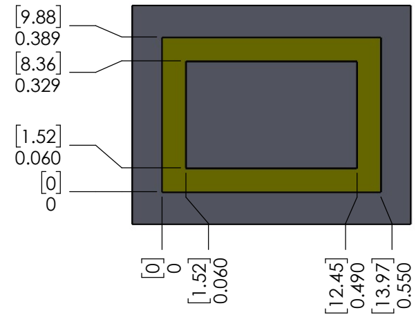
TRACE PATTERN SCALE 3:1
