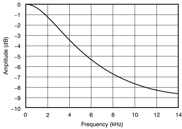
Figure 13. De-emphasis Characteristic
