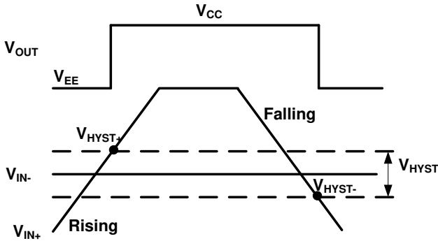
Figure 14. AZV3001A Internal Input Hysteresis Voltage
