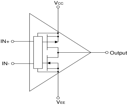
Figure 13. AZV3001A Complementary Output Configuration
