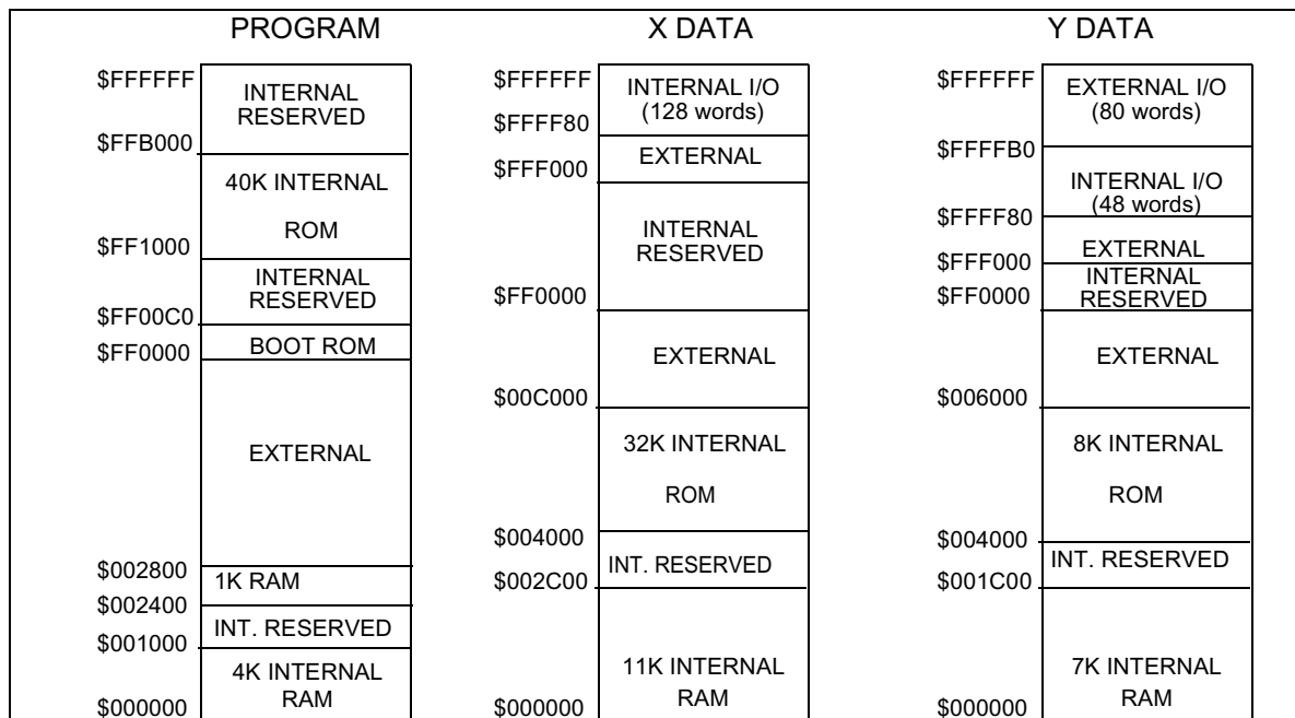
Figure 3-5 Memory Maps for MSW=(1,0), CE=0, MS=1, SC=0
