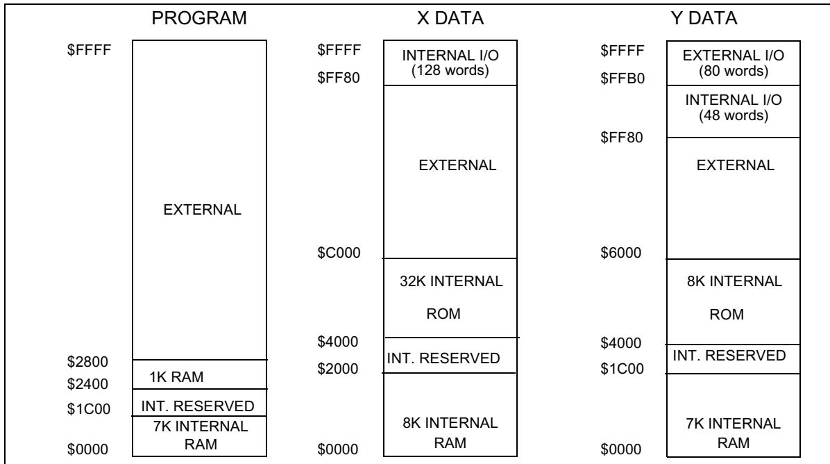
Figure 3-12 Memory Maps for MSW=(0,1), CE=0, MS=1, SC=1
