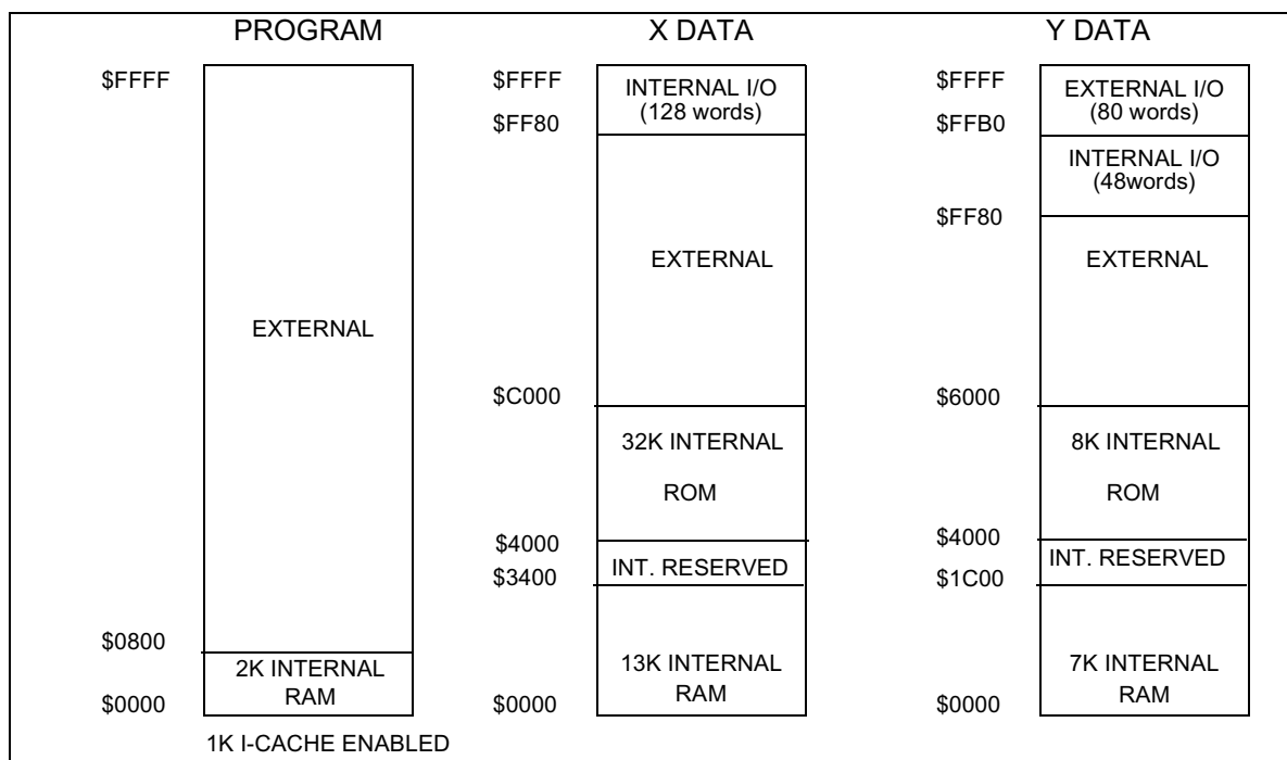
Figure 3-10 Memory Maps for MSW=(X,X), CE=1, MS=0, SC=1
