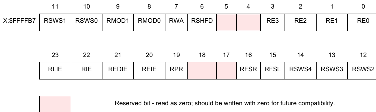
Figure 8-9 RCR Register
