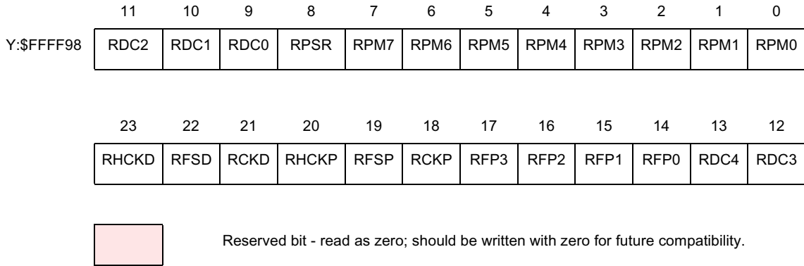
Figure 9-7 RCCR_1 Register
