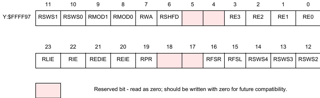
Figure 9-8 RCR_1 Register
