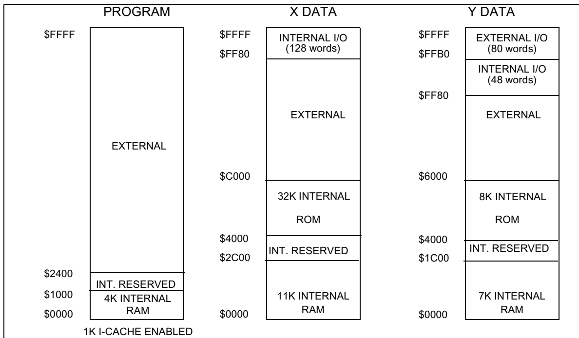
Figure 3-16 Memory Maps for MSW=(1,0), CE=1, MS=1, SC=1
