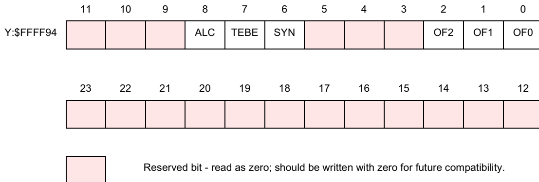
Figure 9-9 SAICR_1 Register
