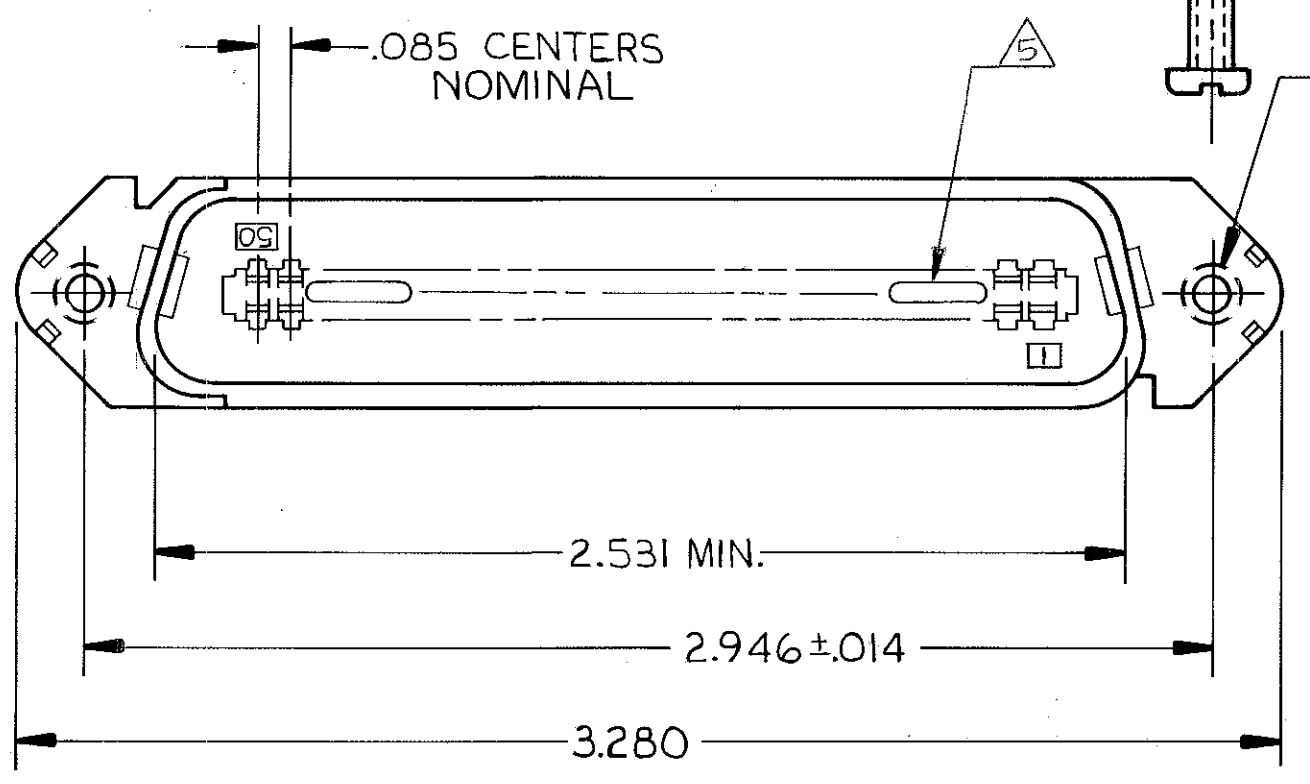
4-40 UNC-2B 2 HOLES
