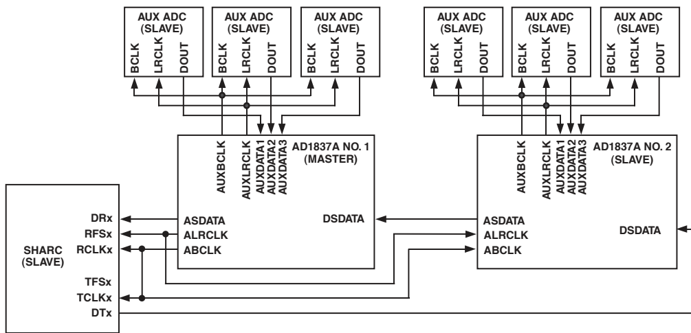
Figure 14. AD1837A Cascade
