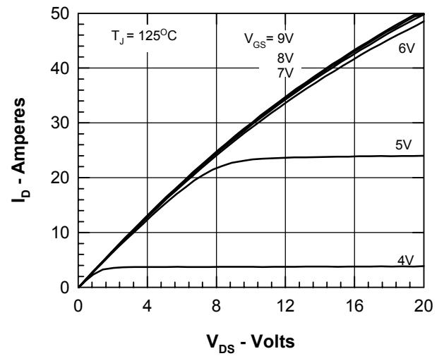
Figure 2. Output Characteristics at 125°C
