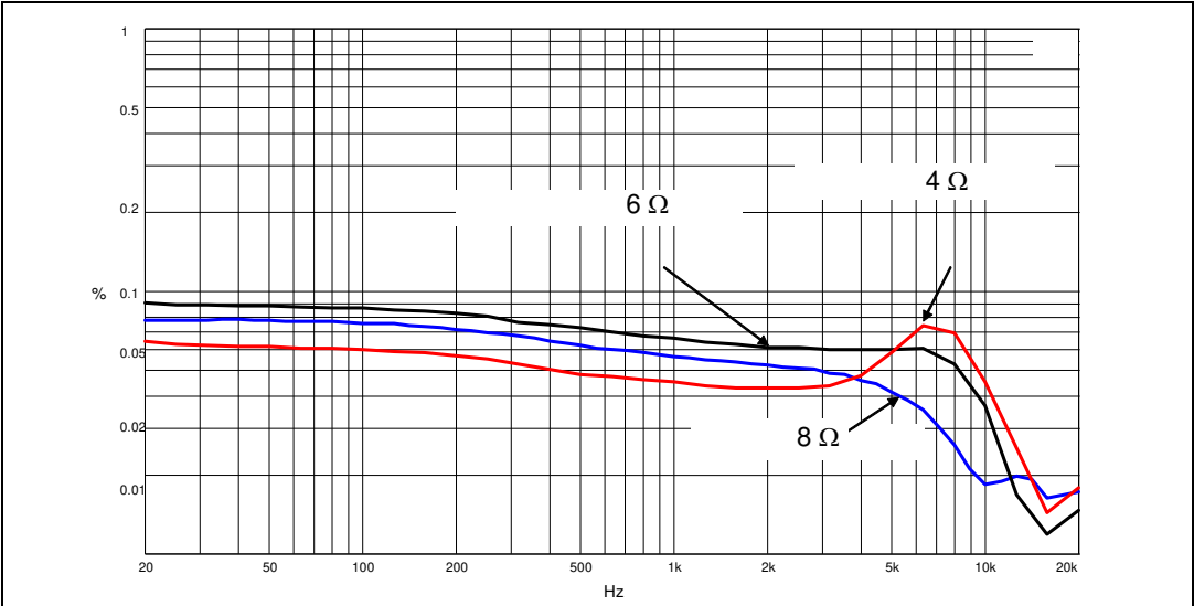
Figure 17. THD vs. frequency ( V_{CC} = 12 V, P_o = 1 W )
