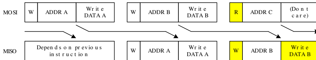
Figure 11 • SPI Read Following Write
