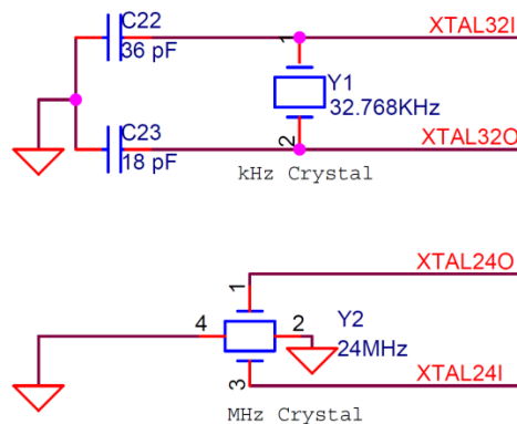
Figure 4-18. Crystal Circuit
