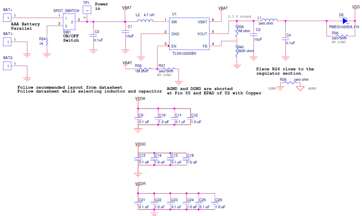
Figure 4-6. Power Supply
