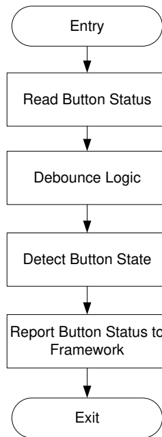
Figure 5-27. Button Subsystem Flow Chart
