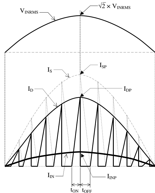
Figure 9-1. Ideal Current Waveform
