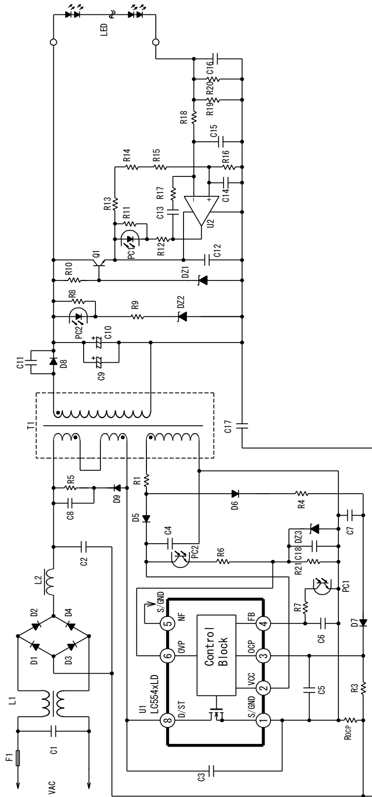
Figure 5-1. Typical Application
