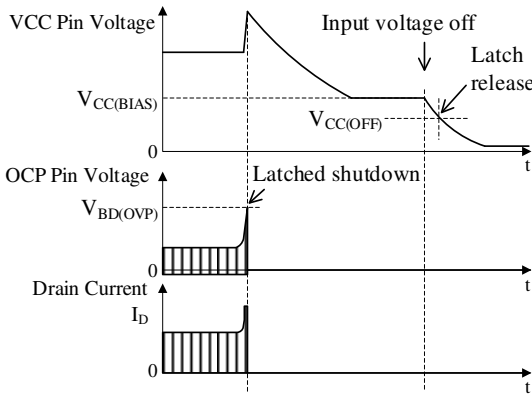
Figure 8-20. OCP_OVP Operational Waveforms
