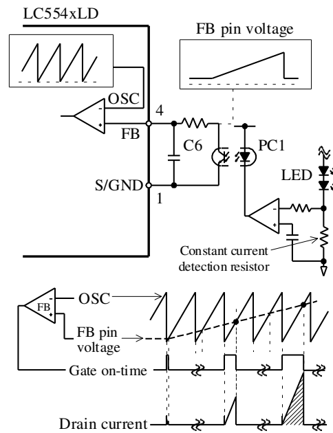
Figure 8-10. On-time Control
