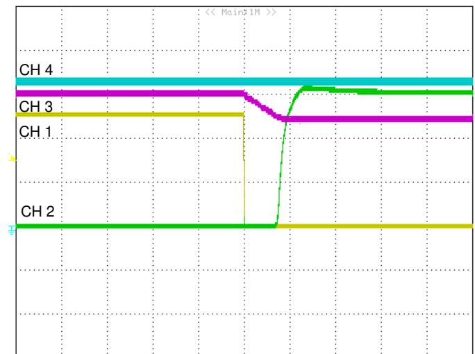
Figure 4: Oring for one feed loss (500μS/div): CH1: inA (2A/div) CH2: inB (2A/div). CH3: VRTN_OUT reference to -48V_OUT (10V/div). CH4: VMGMT_PWR (1V/div).
