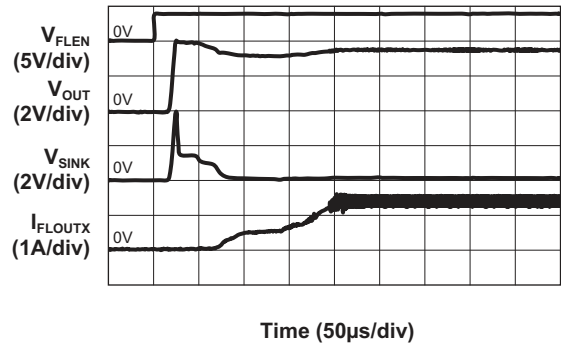
Flash Turn On Characteristic ( I_{FLOUTX} = 750\text{mA}/\text{ch} ; V_{IN} = 3.6\text{V} ; L = 1\mu\text{H} )
