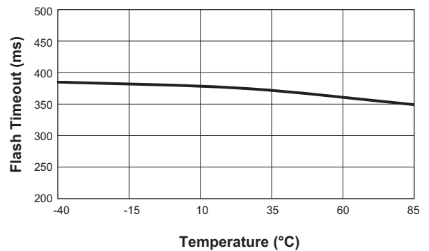
Flash Timeout vs. Temperature ( I_{FLOUTX} = 750\text{mA}/\text{ch} ; V_{IN} = 3.6\text{V} ; C_T = 47\text{nF} )
