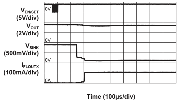
Movie Mode Turn On Characteristic ( I_{FLOUTX} = 103\text{mA}/\text{ch} ; V_{IN} = 3.6\text{V} ; L = 1\mu\text{H} )
