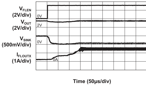
Movie Mode to Flash Turn On Characteristic ( I_{FLOUTX} = 103\text{mA} to 750\text{mA}/\text{ch} ; V_{IN} = 3.6\text{V} ; L = 1\mu\text{H} )
