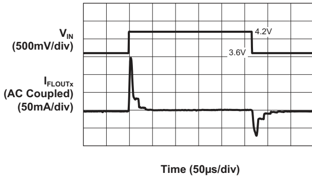
Movie Mode Line Transient ( I_{FLOUTX} = 103\text{mA}/\text{ch} ; V_{IN} = 4.2\text{V} to 3.6\text{V} )
