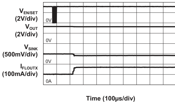
Movie Mode Transition Characteristic ( I_{FLOUTX} = 103\text{mA} to 188\text{mA}/\text{ch} ; C_{OUT} = 0.22\mu\text{F} ; V_{IN} = 3.6\text{V} ; L = 1\mu\text{H} )
