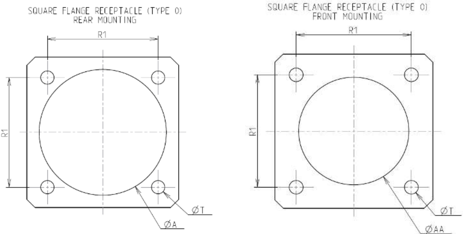
Panel Cutout
