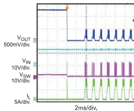
Short-Circuit Entry
