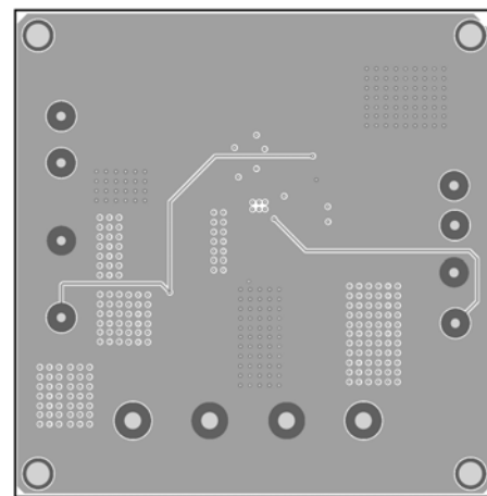
Figure 4—Inner 2 Layer
