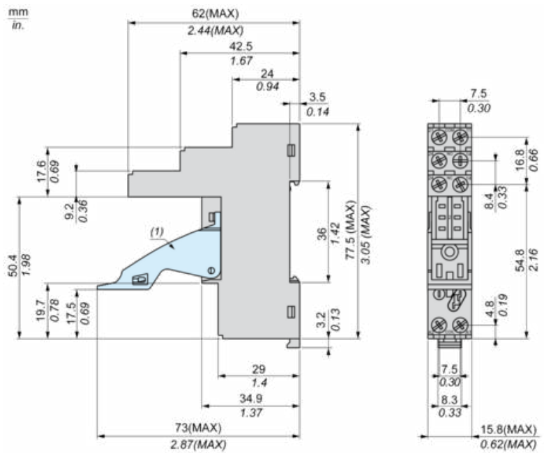
(1) Maintaining clamp
