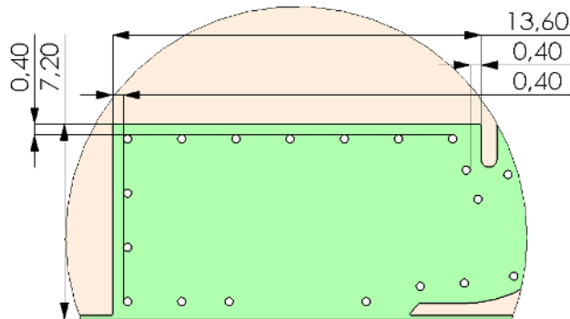
DETAIL C
