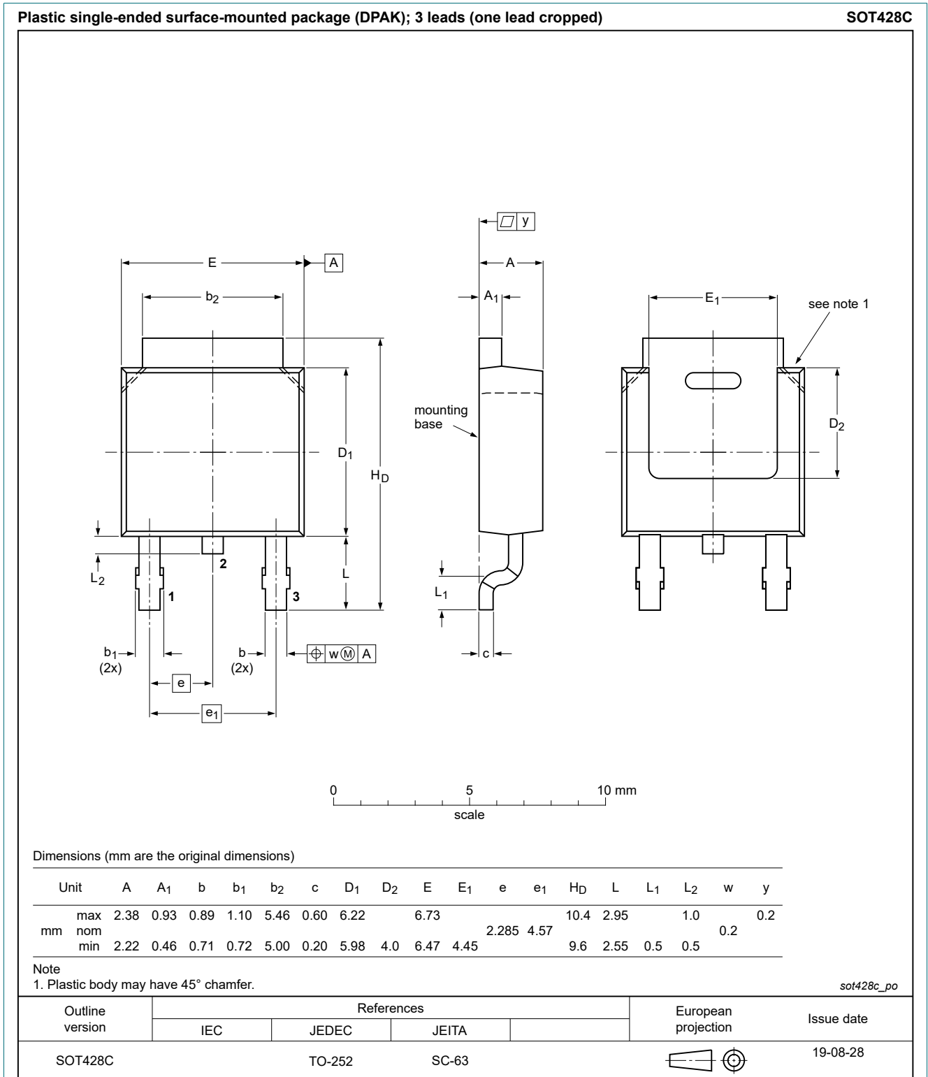
Fig. 12. Package outline DPAK (SOT428C)
