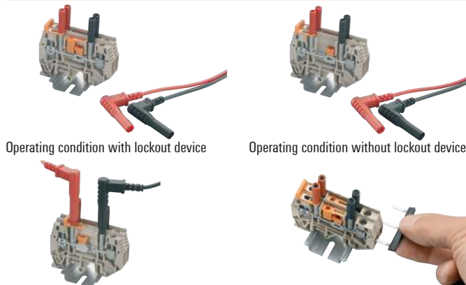
Operating condition with lockout device
