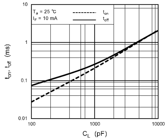
Fig. 12.8 t on , t off - C L
