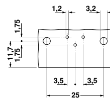
Drilling diagram: VS-PSC 1,5/3-M (-PE)
