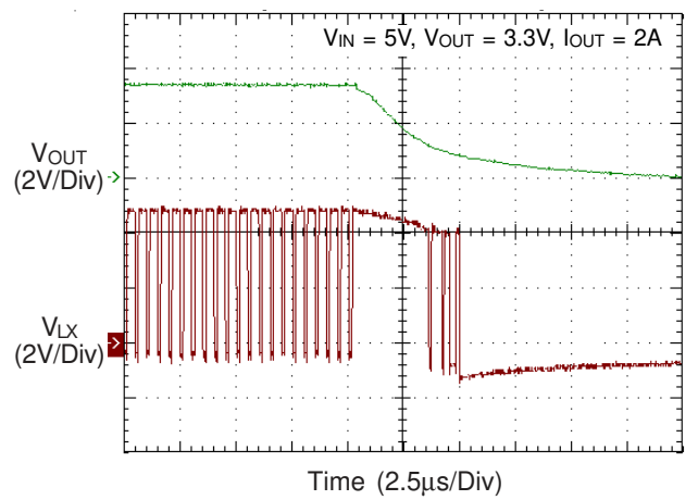
UVP Shutdown
