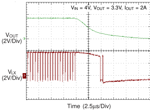
UVP Shutdown
