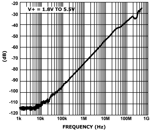
FIGURE 18. OFF-ISOLATION
