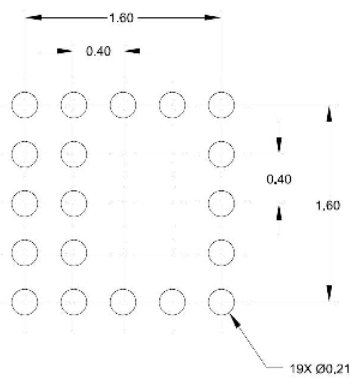
Figure 58 - Outline Drawing - CSP
