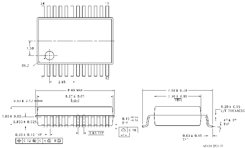
24-Lead Shrink Small Outline Package (SSOP), EIAJ TYPE II, 5.3mm Wide Package Number M2424
