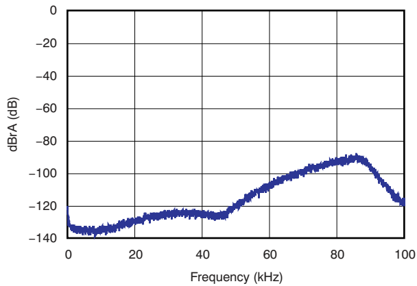
Figure 11. Idle Noise FFT Spectrum (Digital Input)
