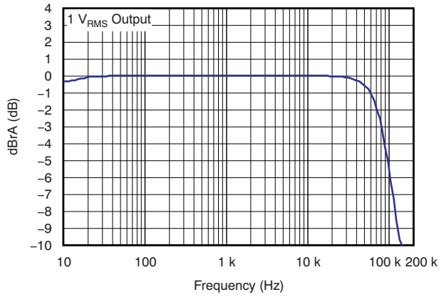
Figure 14. Frequency Response (Analog Input)
