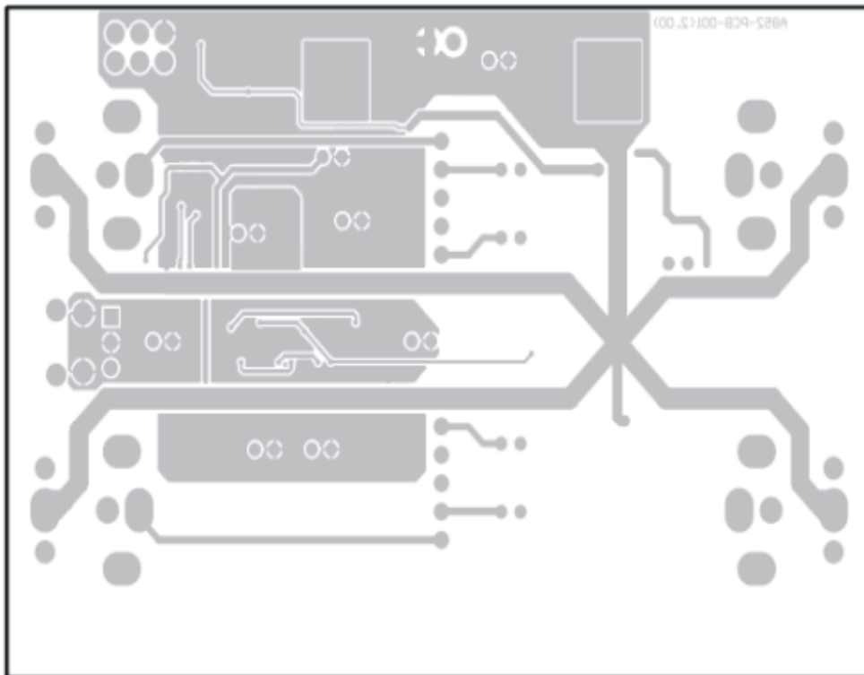
Figure 24. DRV603EVM PCB Bottom Layer
