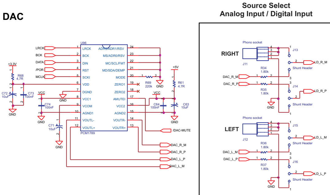
Figure 19. DRV603EVM Schematic: Digital-to-Analog Converter and Source Select
