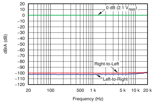
Figure 13. Channel Separation (Digital Input)
