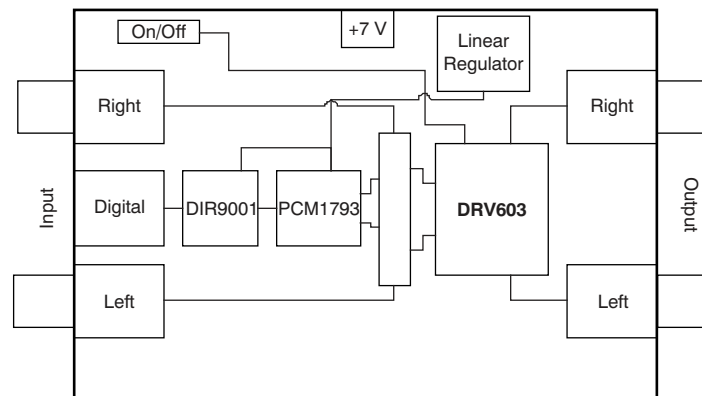
Figure 1. DRV603EVM Functional Block Diagram
