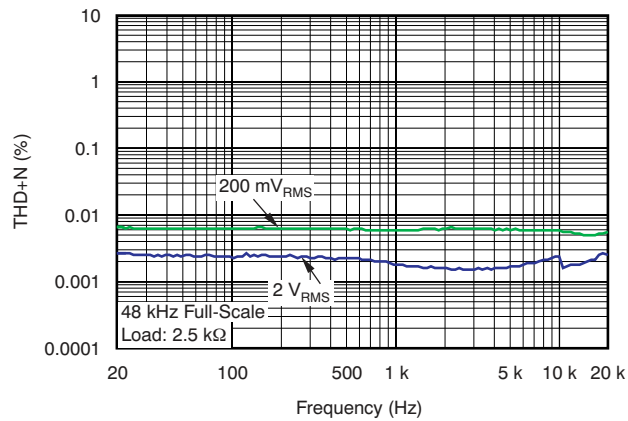
Figure 7. THD+N versus Frequency (Digital Input, 0 dBFS)
