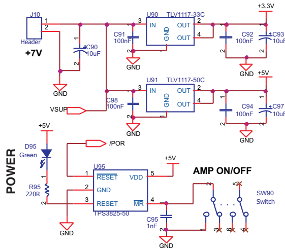
Figure 21. DRV603EVM Schematic: TOSLINK and Power Supply
