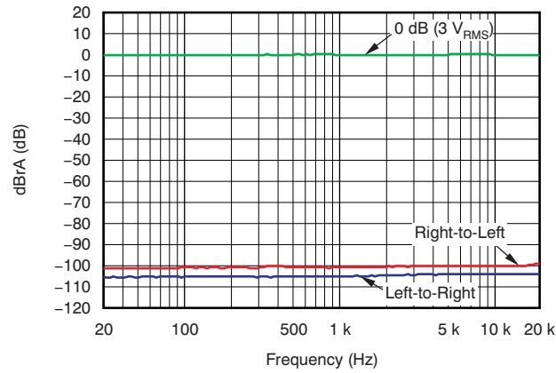
Figure 12. Channel Separation (Analog Input)
