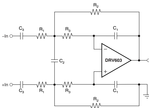
Figure 3. Differential Input, Second-Order, Active Low-Pass Filter
