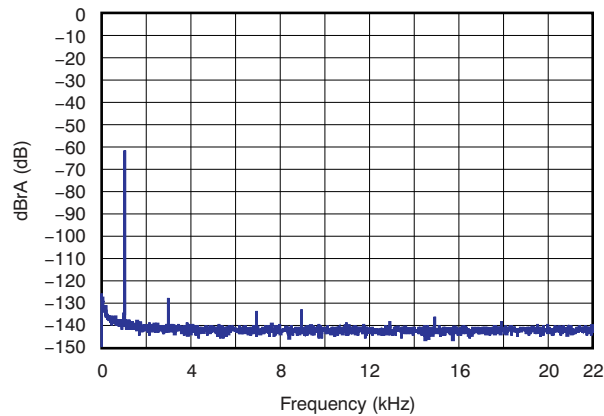
Figure 8. FFT Spectrum with -60-dBFS Tone (Analog Input)
