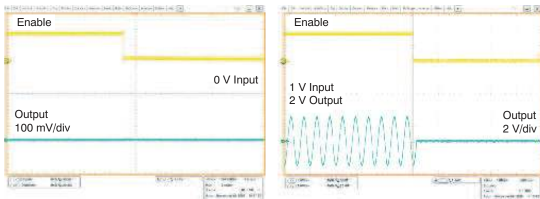
Figure 17. Pop/Click (Disable)
