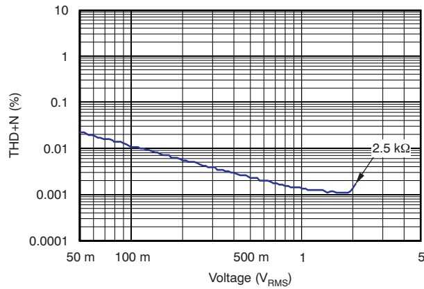
Figure 5. THD+N versus Voltage (Digital Input)
