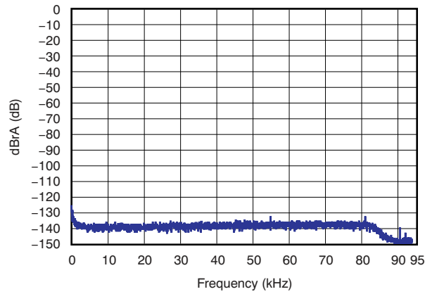
Figure 10. Idle Noise FFT Spectrum (Analog Input)
