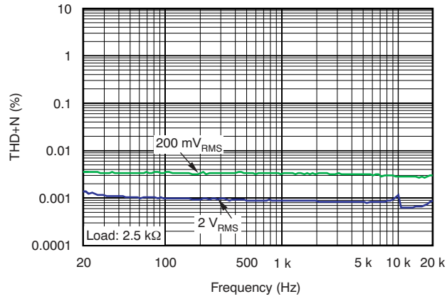
Figure 6. THD+N versus Frequency (Analog Input)
