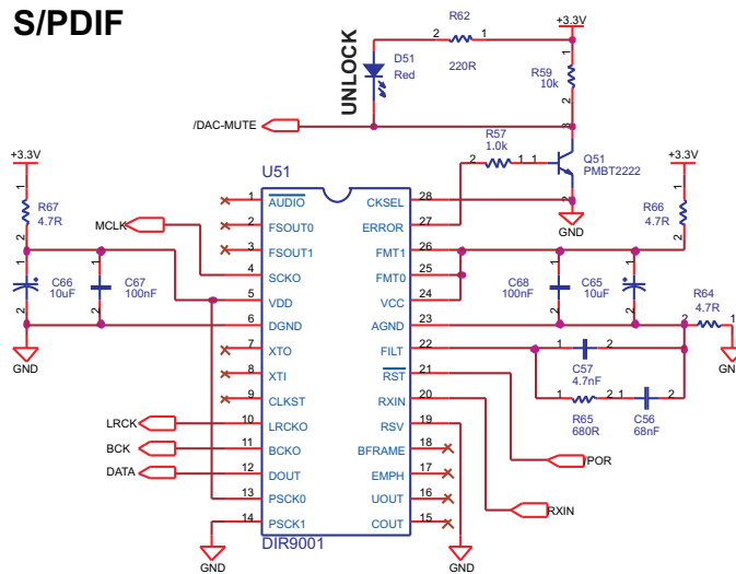
Figure 20. DRV603EVM Schematic: S/PDIF Receiver
