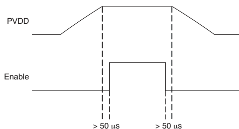
Figure 2. Power-Up/-Down Sequence
