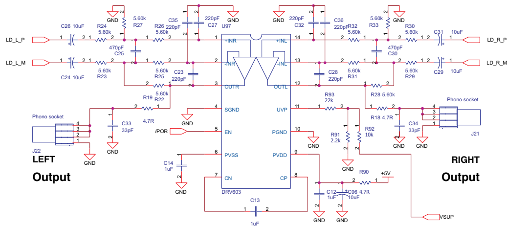
Figure 18. DRV603EVM Schematic: DRV603
