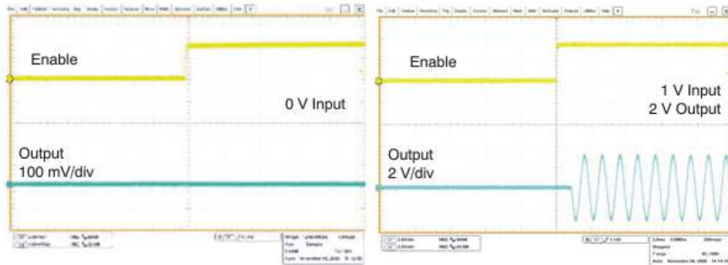
Figure 16. Pop/Click (Enable)
