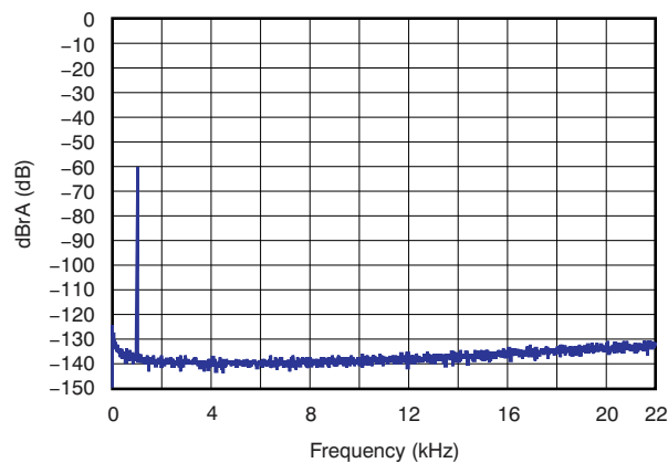
Figure 9. FFT Spectrum with -60-dBFS Tone (Digital Input)
