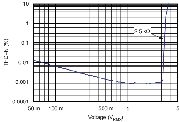
Figure 4. THD+N versus Voltage (Analog Input)
