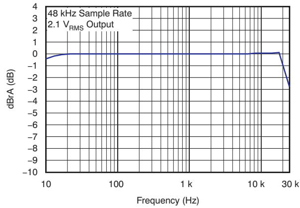
Figure 15. Frequency Response (Digital Input)
