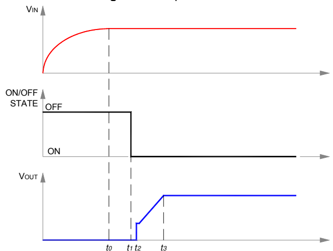
Fig. 8: Start-up scenario #2.
