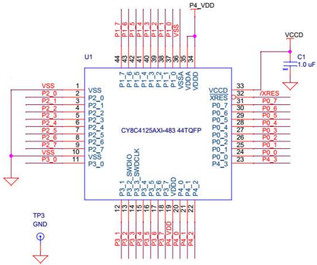
Figure A-2. CY8C4125AXI-483 (CY8CKIT-049-41XX only)
