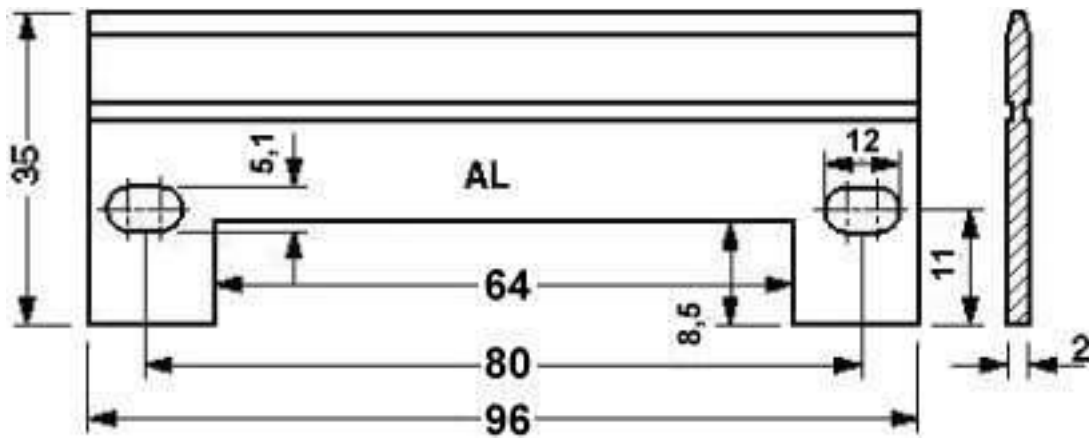
Dimensioned drawing
