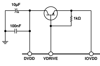
Figure 20. External Components Required for Voltage Regulator Circuit
