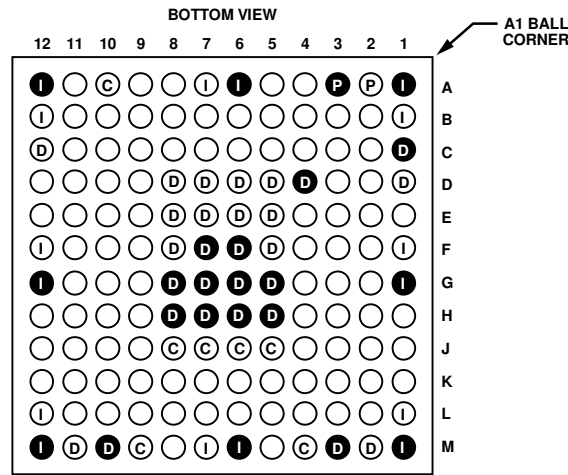
Figure 12. Ball Configuration, Bottom View (Not to Scale)
